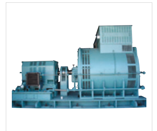
10MVA MG Set for test equipment of electric power machinery
