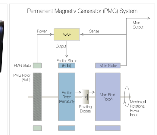
Schematic diagram (PMG)
