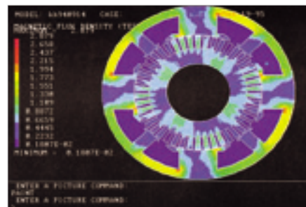
Magnetic Flux Density in core
